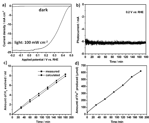
Figure 3. a) Current–potential curves, and b) chronoamperometry of the \text{Pt}/\text{TiO}_2/\text{Ti}/\text{n}^+\text{p-Si} electrode at an applied potential of 0.2 V vs. RHE in a three-electrode system. c) The amount of gas evolved from the photocathode compartment. ■ represents the values measured and ● represents the values calculated from the photocurrent. d) The rate of \text{Fe}^{3+} generation based upon the UV/Vis absorption spectra analysis. Electrolyte: 0.2 M \text{FeSO}_4 acidic solution. Light source: AM1.5G, 100 \text{ mW cm}^{-2} .
