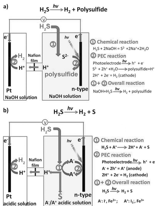
Scheme 1. a) Conventional photoelectrochemical approach, and b) proposed photoelectrochemical-chemical loop for \text{H}_2\text{S} splitting on a n-type photoelectrode linked with redox couples.
